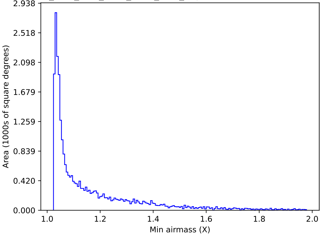
ddf_acor_sf10_lsf30_lsr20_v3.4_10yrs Yr 1 i band: Min airmass
