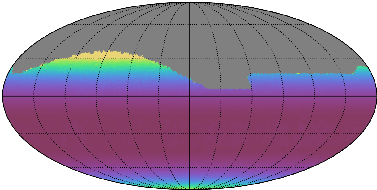
ddf_acor_sf10_lsf30_lsr20_v3.4_10yrs Yr 1 all bands: Min airmass
