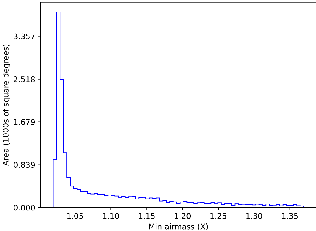
ddf_acor_sf10_lsf30_lsr20_v3.4_10yrs WFD z band: Min airmass
