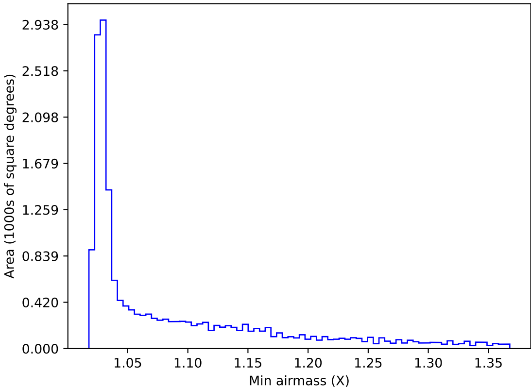
ddf_acor_sf10_lsf30_lsr20_v3.4_10yrs WFD i band: Min airmass
