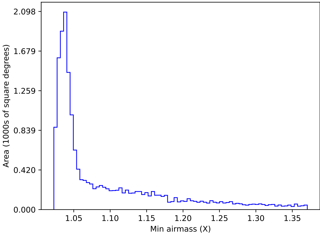
ddf_acor_sf10_lsf30_lsr20_v3.4_10yrs WFD g band: Min airmass
