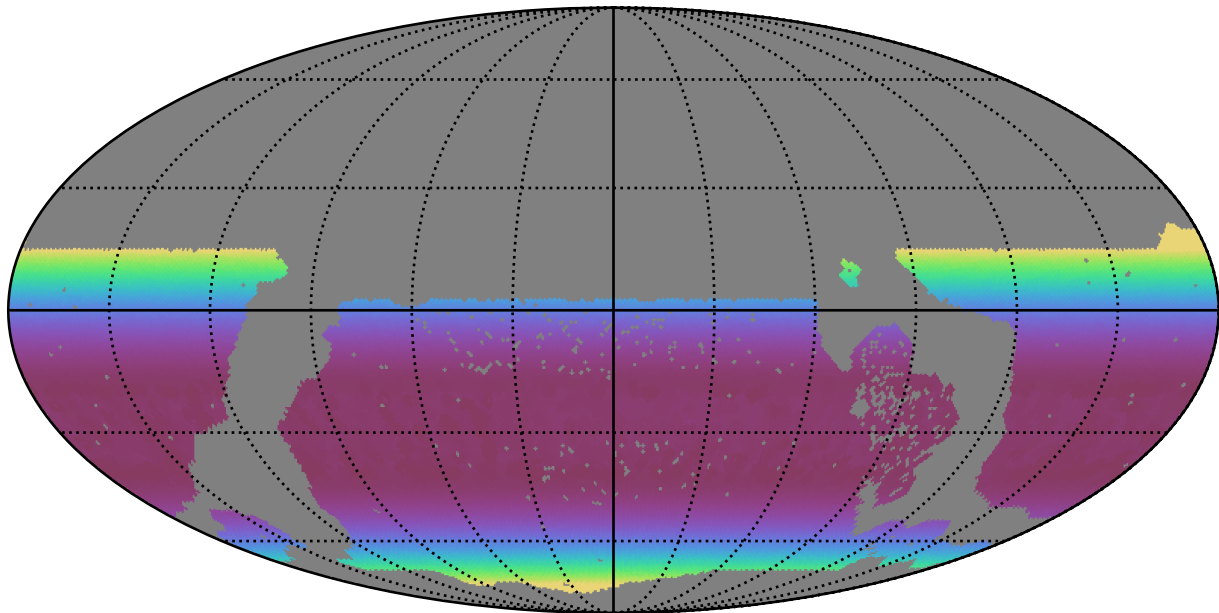
ddf_acor_sf10_lsf30_lsr20_v3.4_10yrs WFD all bands: Min airmass
