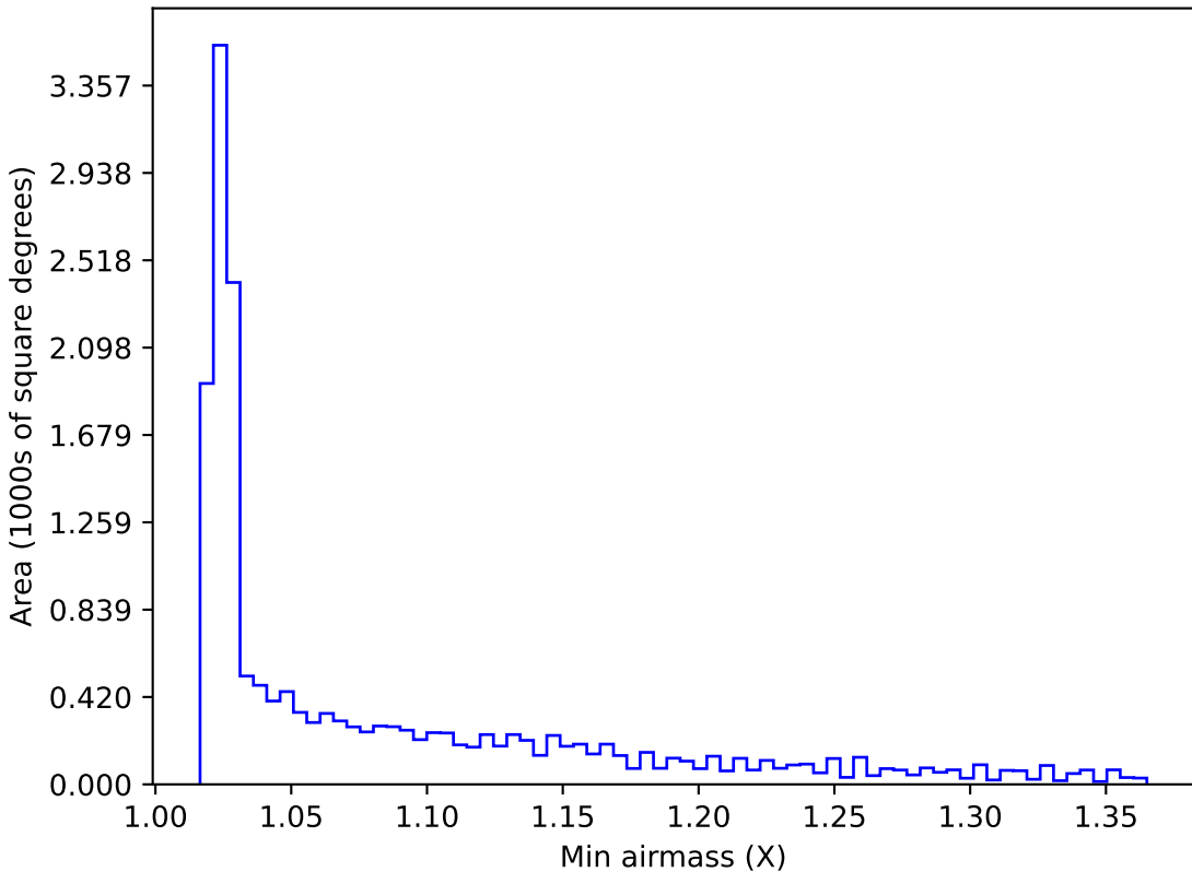
ddf_acor_sf10_lsf30_lsr20_v3.4_10yrs WFD all bands: Min airmass
