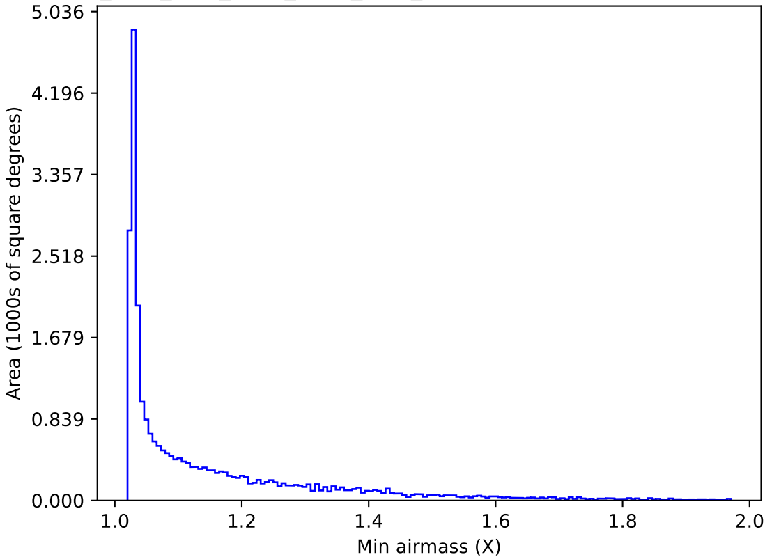
ddf_acor_sf10_lsf30_lsr20_v3.4_10yrs All sky z band: Min airmass
