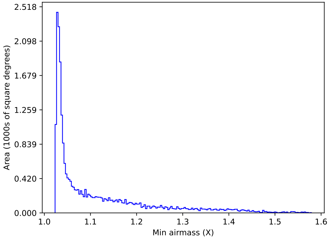
ddf_acor_sf10_lsf30_lsr20_v3.4_10yrs All sky y band: Min airmass
