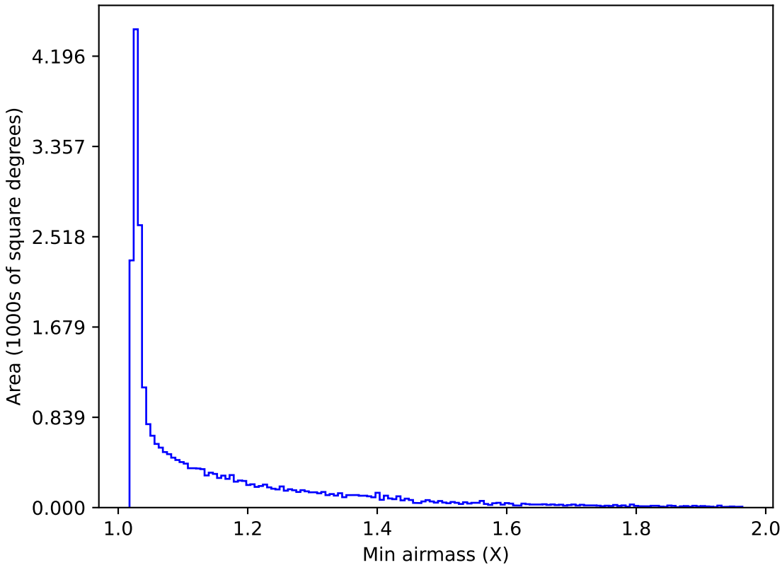
ddf_acor_sf10_lsf30_lsr20_v3.4_10yrs All sky r band: Min airmass
