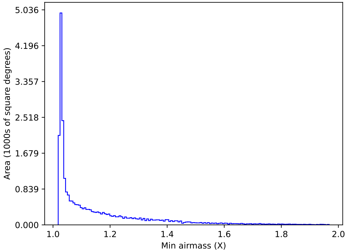
ddf_acor_sf10_lsf30_lsr20_v3.4_10yrs All sky i band: Min airmass
