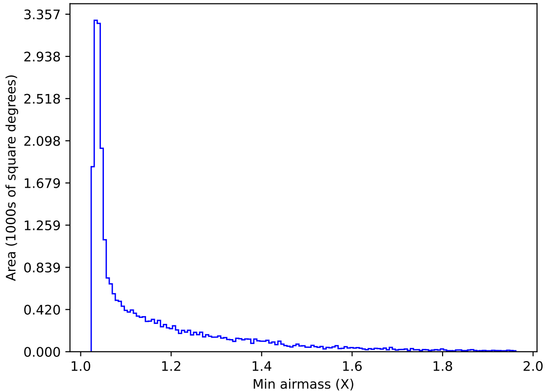
ddf_acor_sf10_lsf30_lsr20_v3.4_10yrs All sky g band: Min airmass
