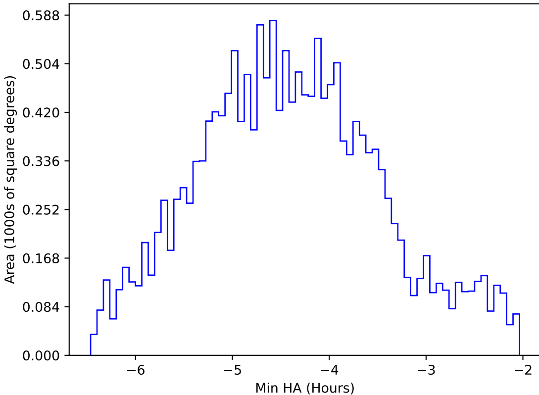
ddf_acor_sf10_lsf30_lsr20_v3.4_10yrs WFD z band: Min HA
