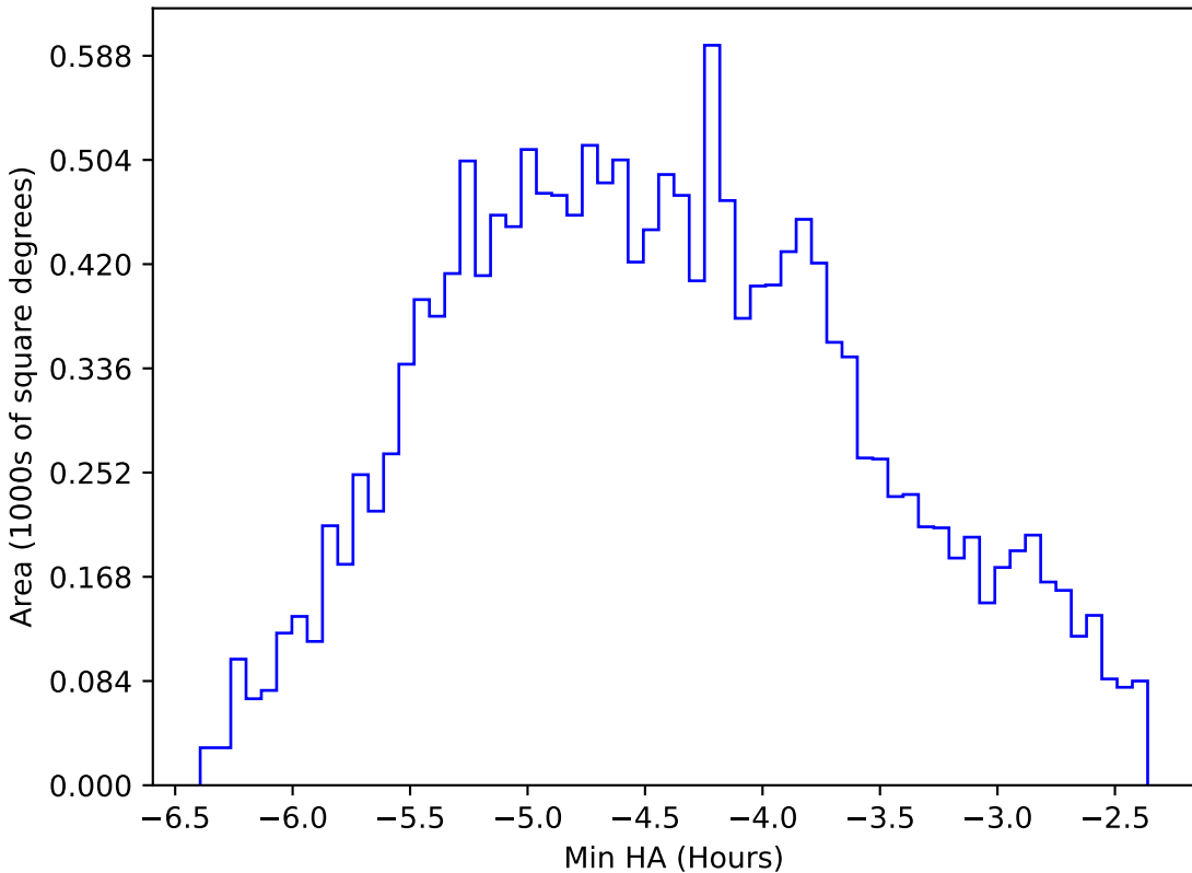
ddf_acor_sf10_lsf30_lsr20_v3.4_10yrs WFD r band: Min HA
