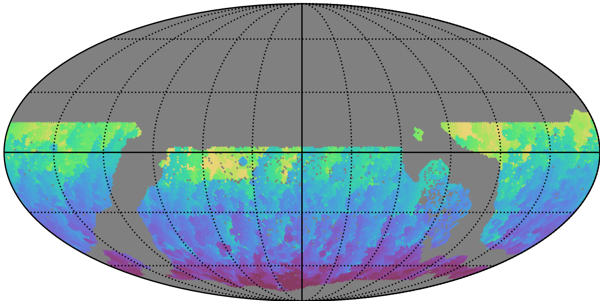
ddf_acor_sf10_lsf30_lsr20_v3.4_10yrs WFD g band: Min HA
