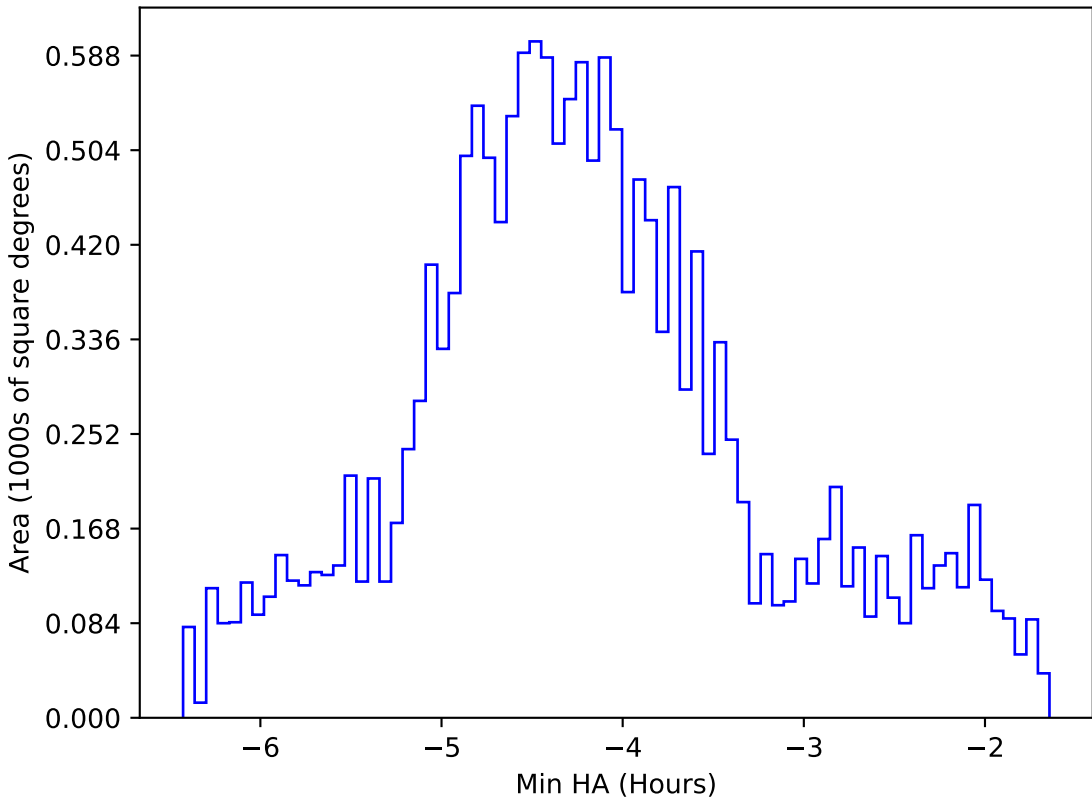
ddf_acor_sf10_lsf30_lsr20_v3.4_10yrs WFD g band: Min HA
