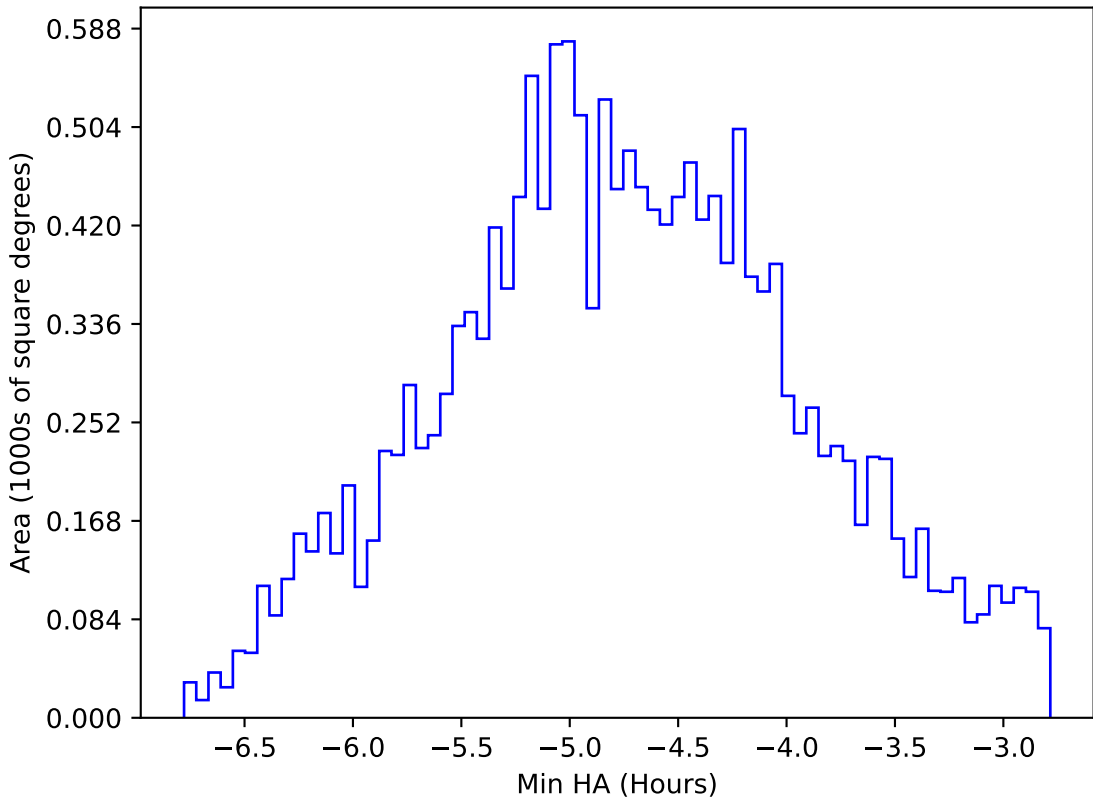
ddf_acor_sf10_ls30_lsr20_v3.4_10yrs WFD all bands: Min HA
