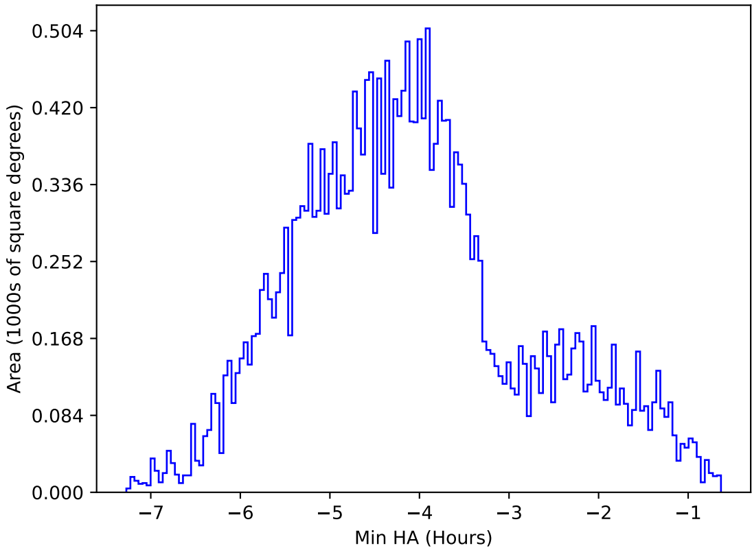
ddf_acor_sf10_lsf30_lsr20_v3.4_10yrs All sky z band: Min HA
