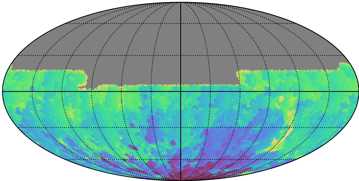
ddf_acor_sf10_lsf30_lsr20_v3.4_10yrs All sky u band: Min HA
