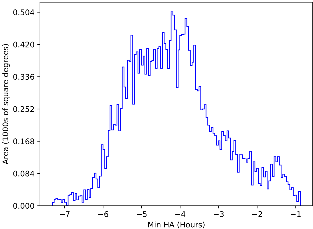
ddf_acor_sf10_ls30_lsr20_v3.4_10yrs All sky r band: Min HA
