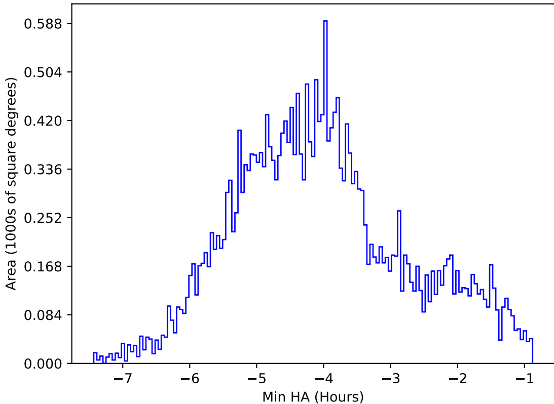
ddf_acor_sf10_ls30_lsr20_v3.4_10yrs All sky i band: Min HA
