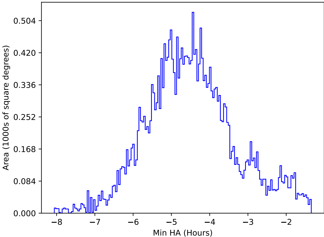
ddf_acor_sf10_lsf30_lsr20_v3.4_10yrs All sky all bands: Min HA
