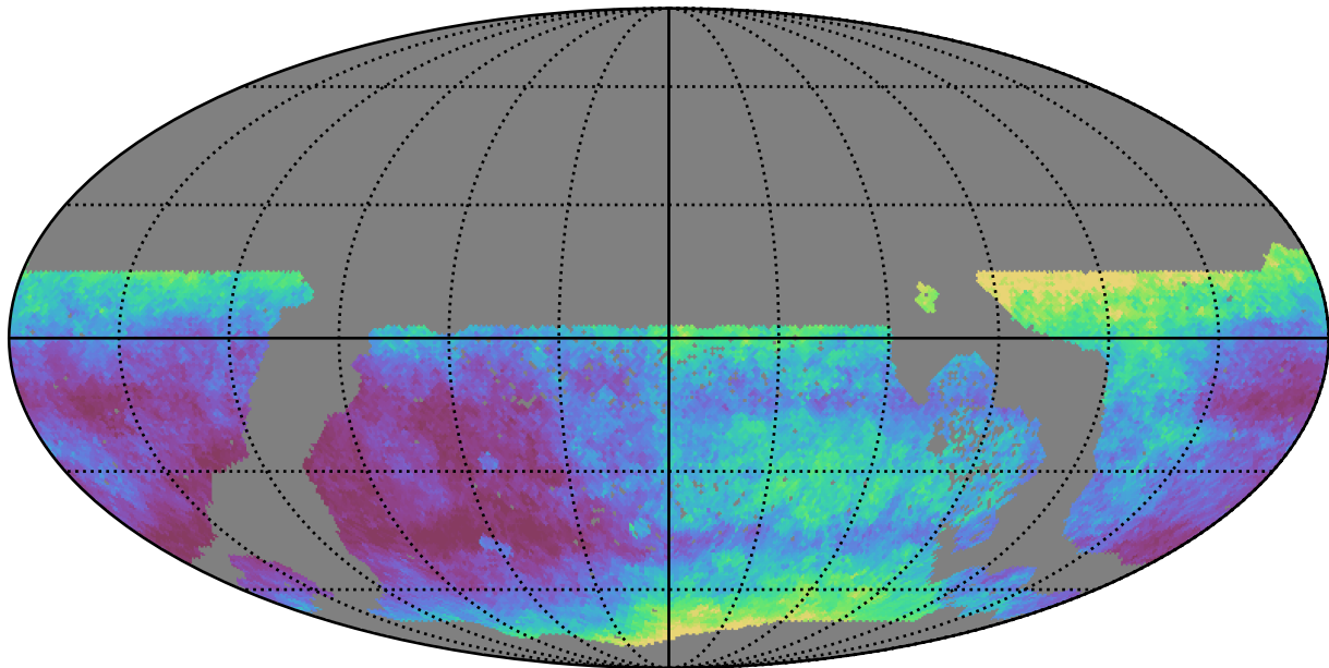
ddf_acor_sf10_lsf30_lsr20_v3.4_10yrs WFD i band: Median seeingEff
