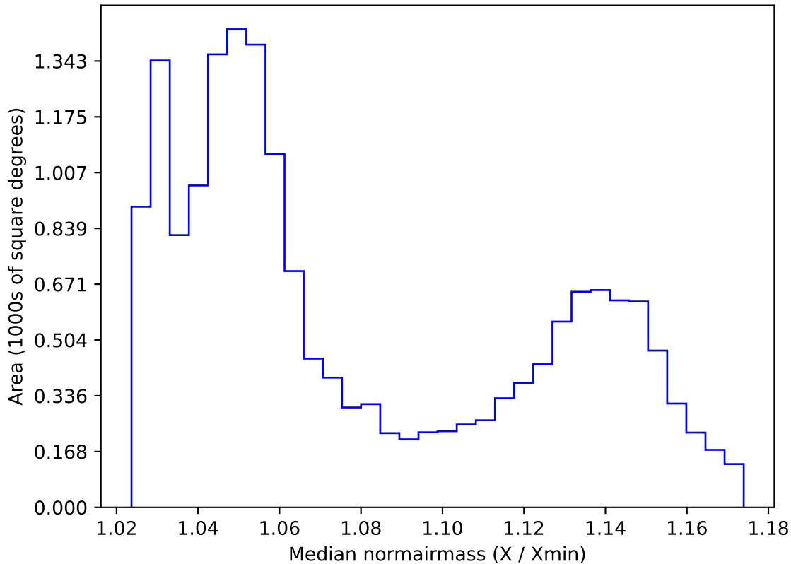
ddf_acor_sf10_lsf30_lsr20_v3.4_10yrs WFD all bands: Median normairmass
