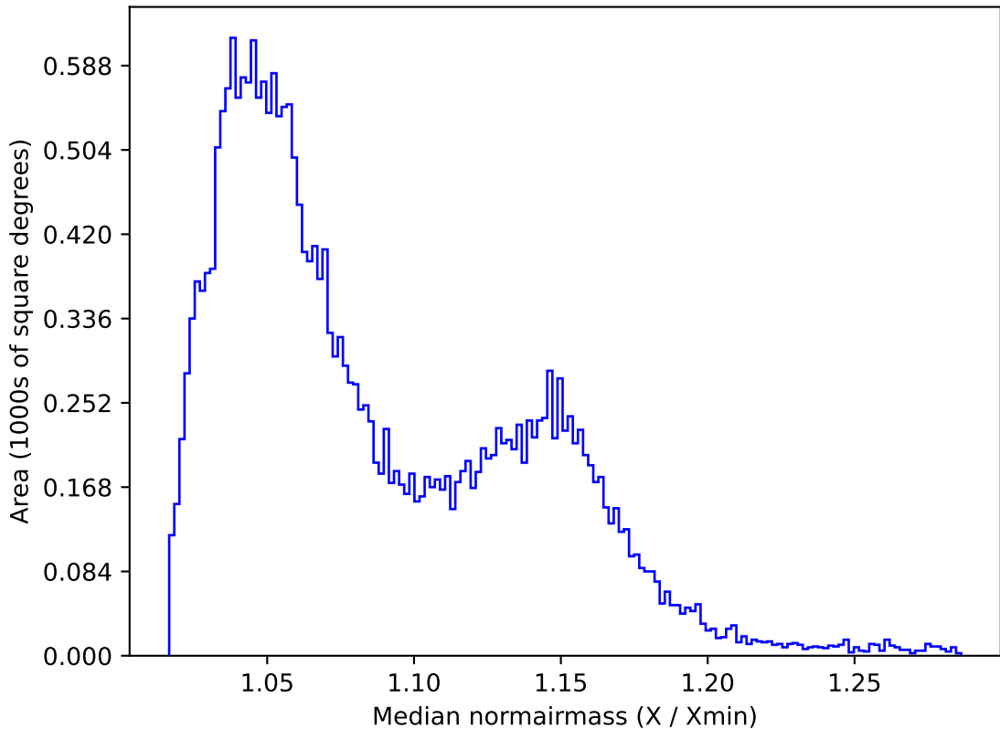
ddf_acor_sf10_lsf30_lsr20_v3.4_10yrs All sky z band: Median normairmass
