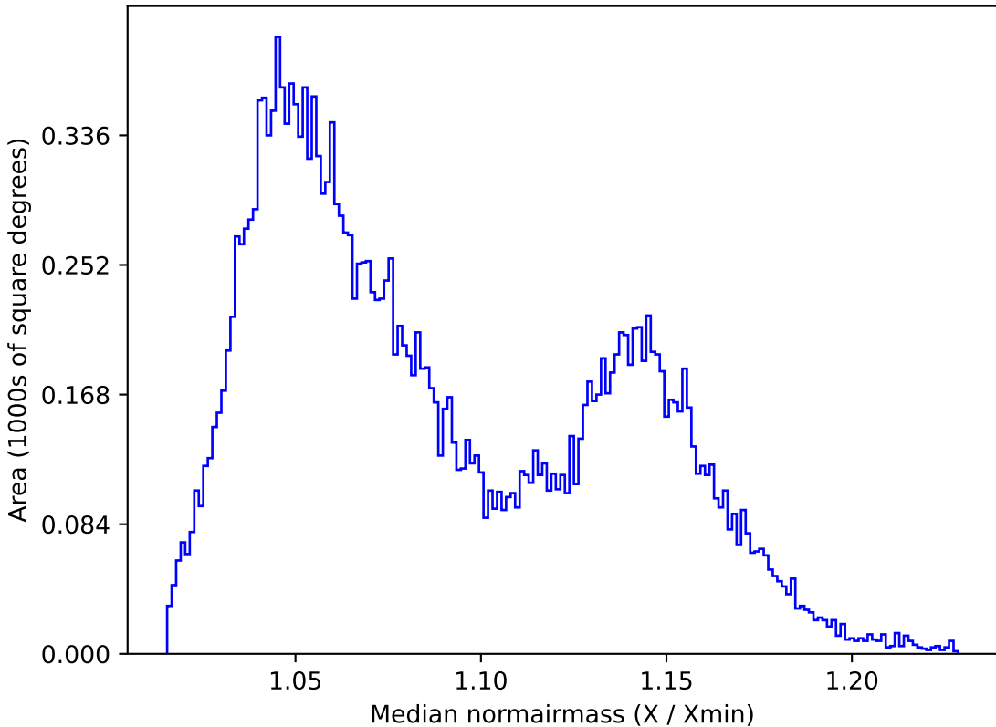
ddf_acor_sf10_ls30_lsr20_v3.4_10yrs All sky y band: Median normairmass
