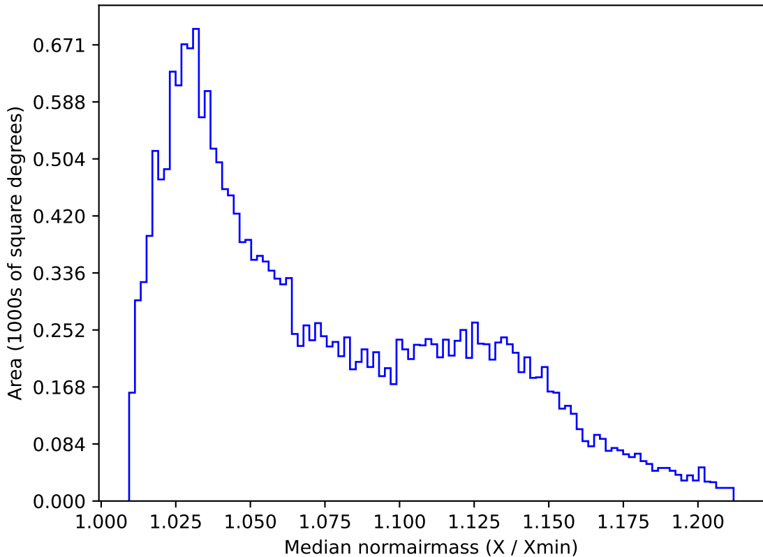
ddf_acor_sf10_lsf30_lsr20_v3.4_10yrs All sky u band: Median normairmass
