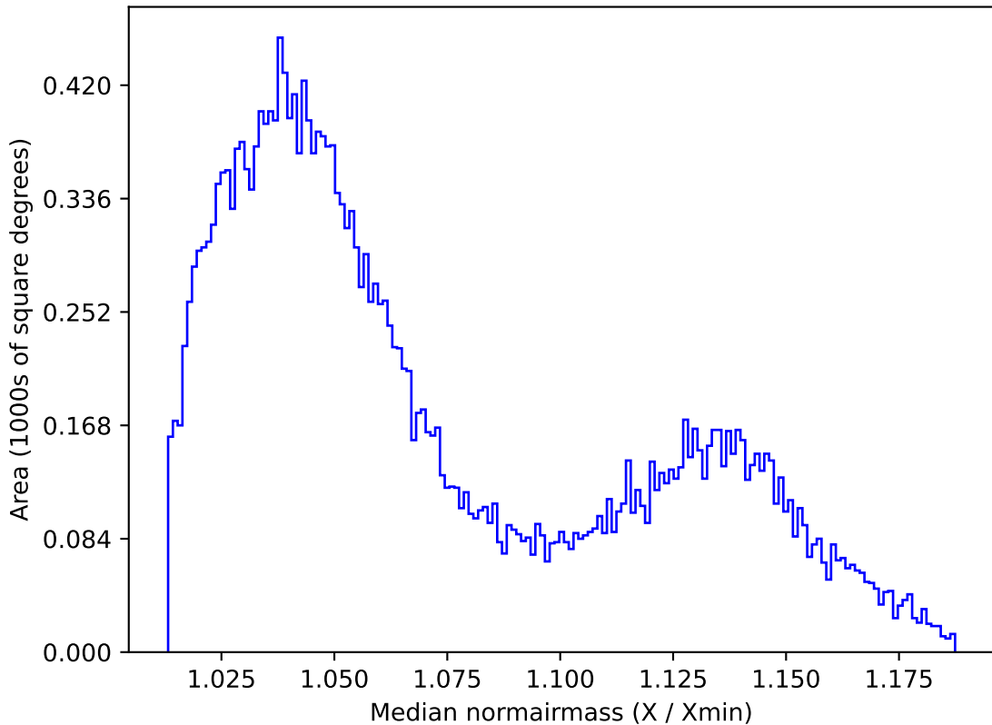
ddf_acor_sf10_ls30_lsr20_v3.4_10yrs All sky r band: Median normairmass
