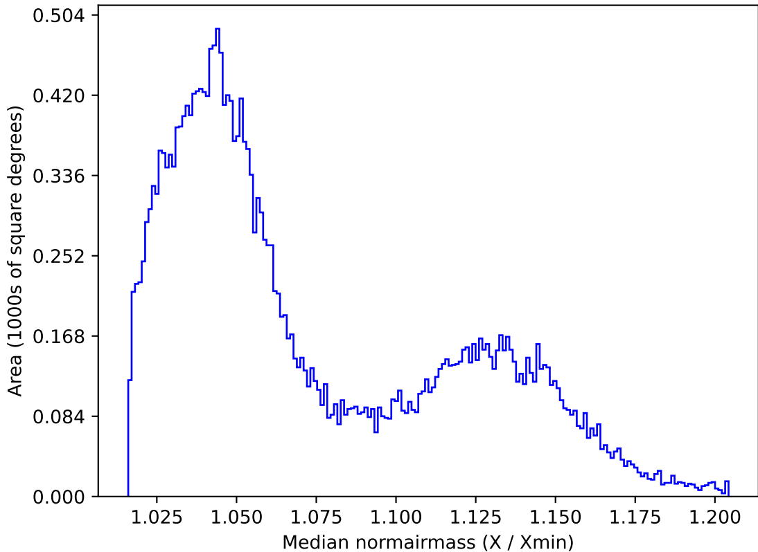
ddf_acor_sf10_lsf30_lsr20_v3.4_10yrs All sky i band: Median normairmass
