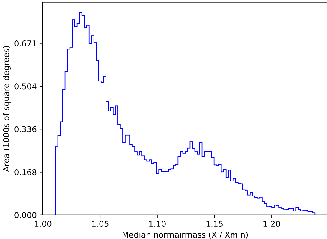
ddf_acor_sf10_ls30_lsr20_v3.4_10yrs All sky g band: Median normairmass
