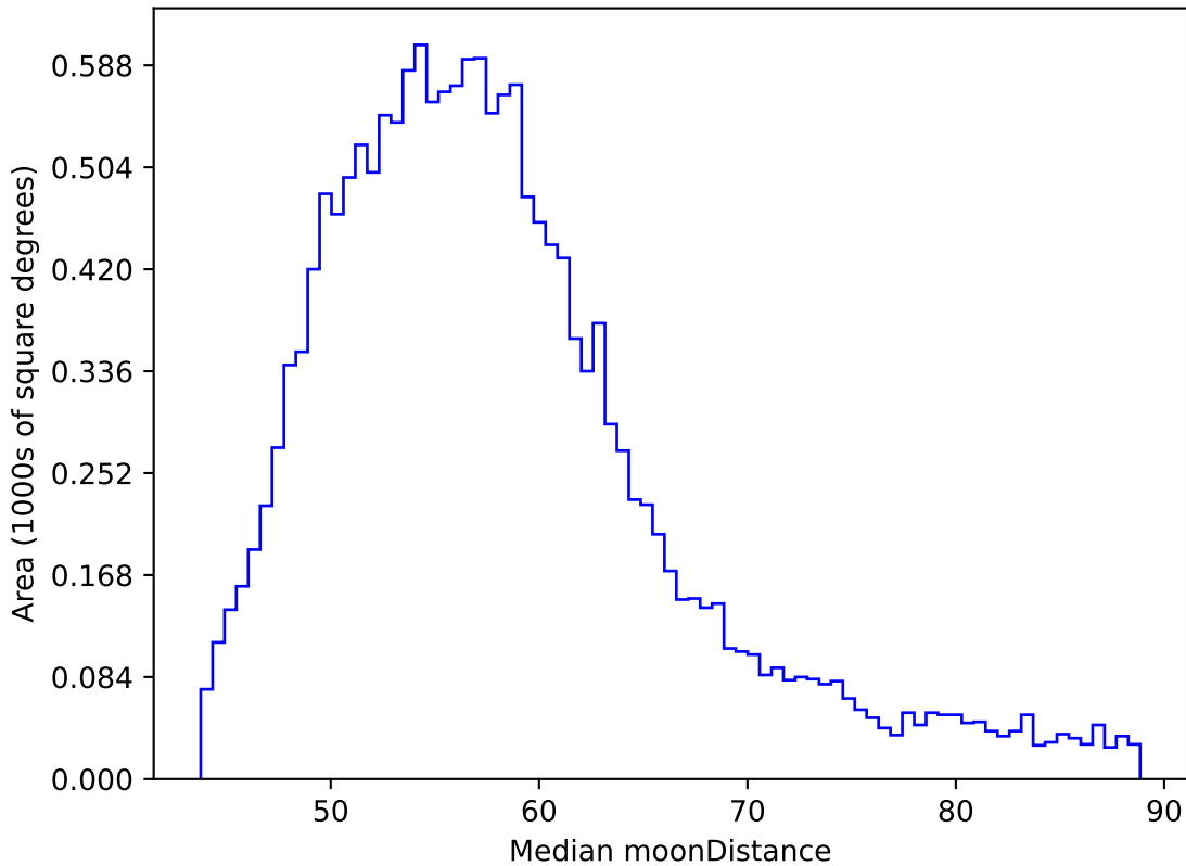
ddf_acor_sf10_lsf30_lsr20_v3.4_10yrs WFD y band: Median moonDistance
