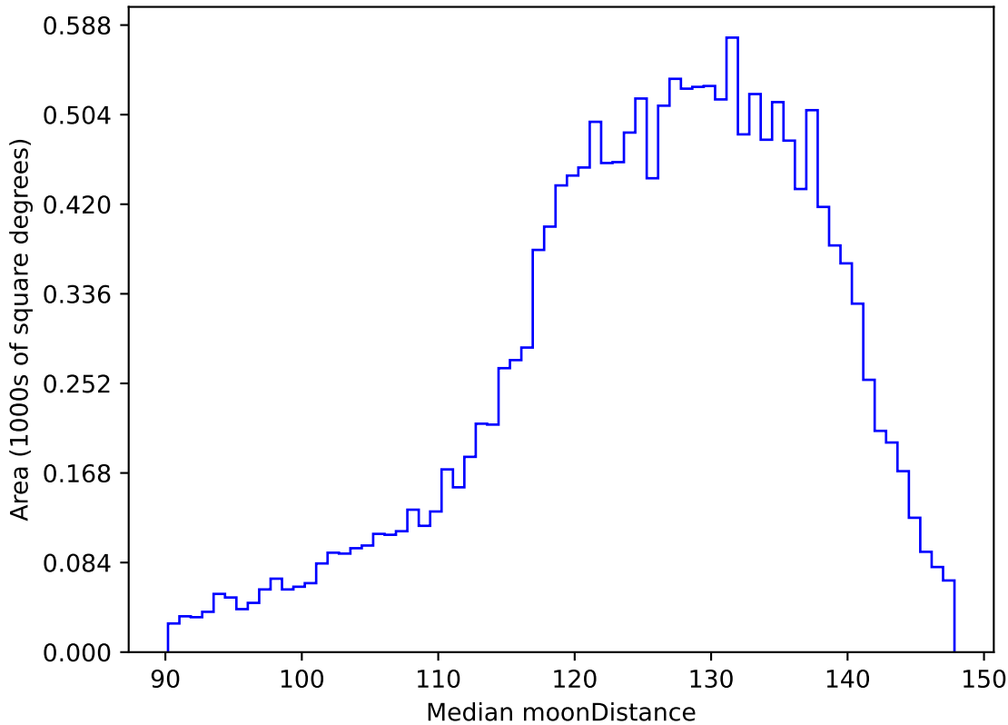
ddf_acor_sf10_lsf30_lsr20_v3.4_10yrs WFD u band: Median moonDistance
