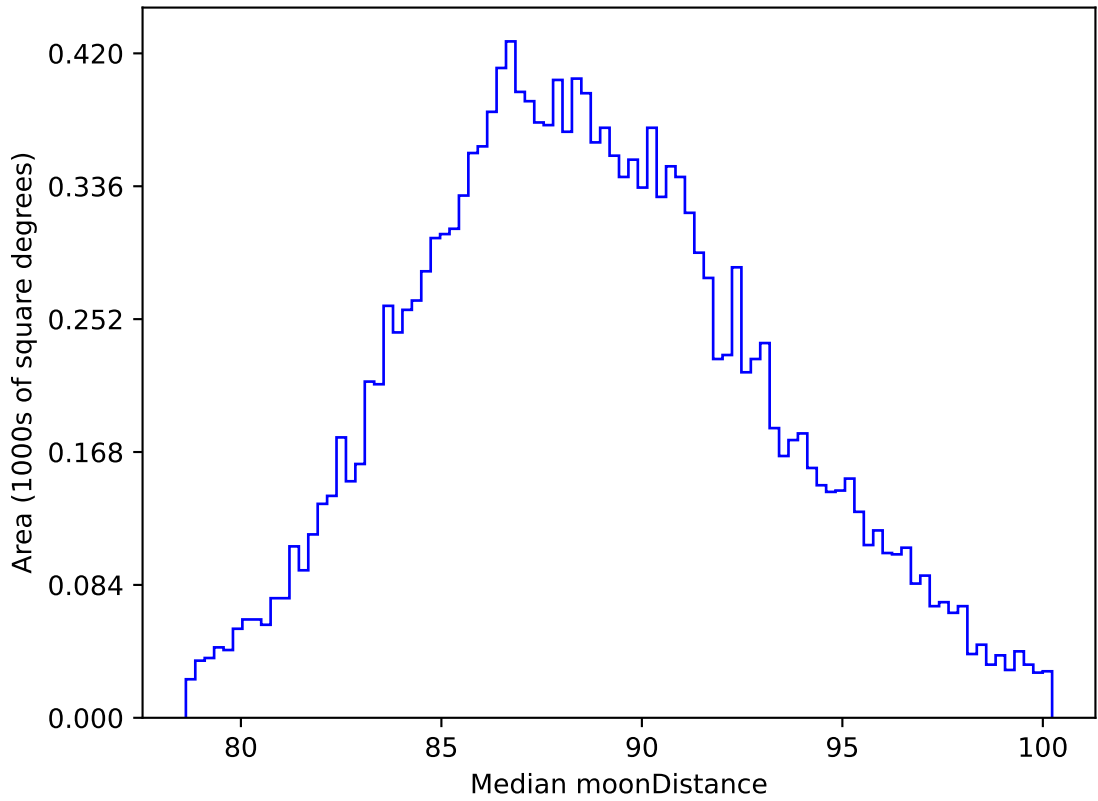
ddf_acor_sf10_lsf30_lsr20_v3.4_10yrs WFD all bands: Median moonDistance
