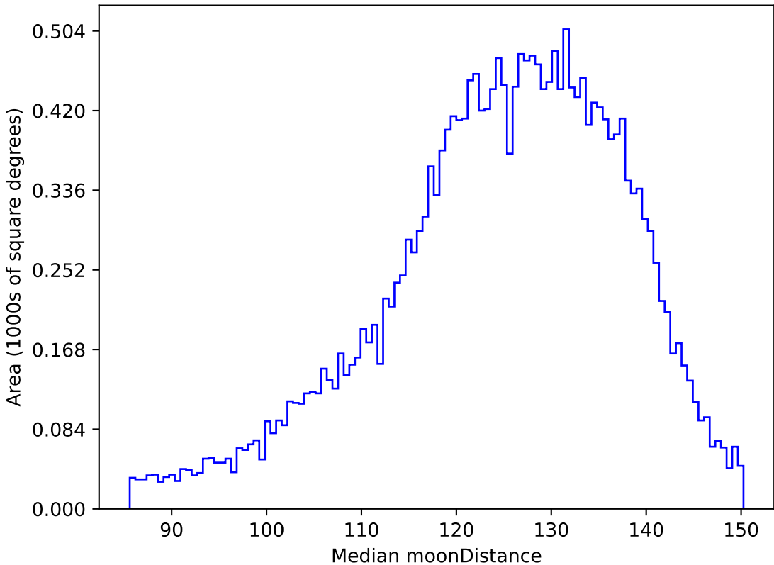
ddf_acor_sf10_lsf30_lsr20_v3.4_10yrs All sky u band: Median moonDistance
