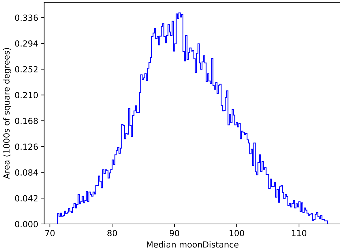
ddf_acor_sf10_lsf30_lsr20_v3.4_10yrs All sky i band: Median moonDistance
