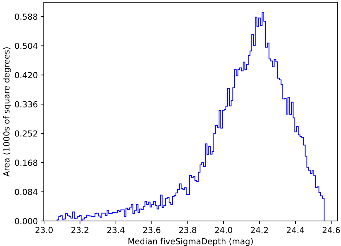
ddf_acor_sf10_lsf30_lsr20_v3.4_10yrs Yr 1 r band: Median fiveSigmaDepth
