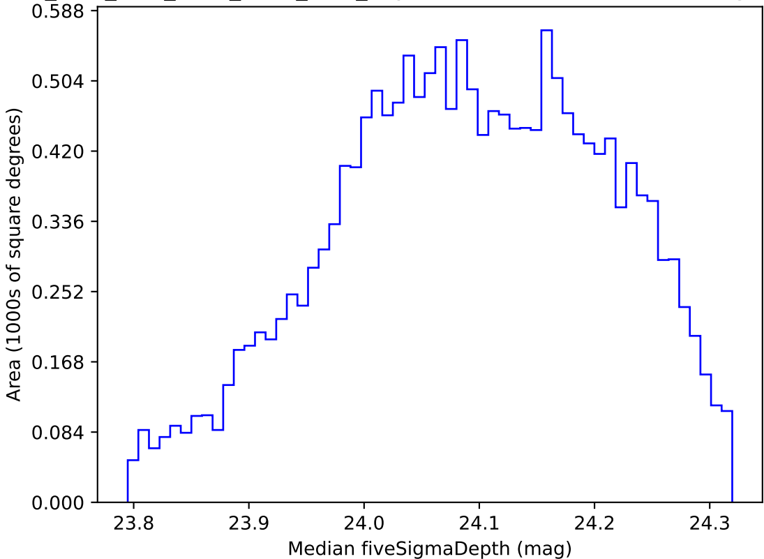
ddf_acor_sf10_lsf30_lsr20_v3.4_10yrs WFD r band: Median fiveSigmaDepth
