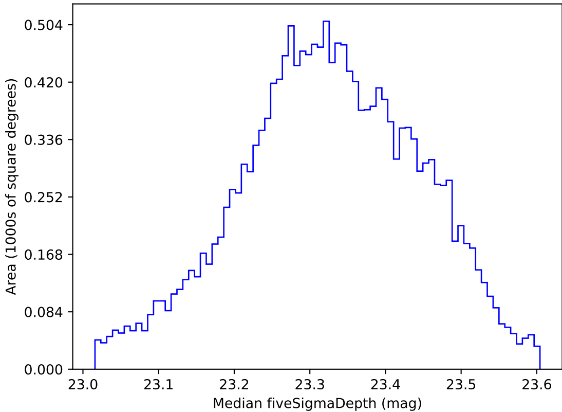
ddf_acor_sf10_lsf30_lsr20_v3.4_10yrs WFD all bands: Median fiveSigmaDepth
