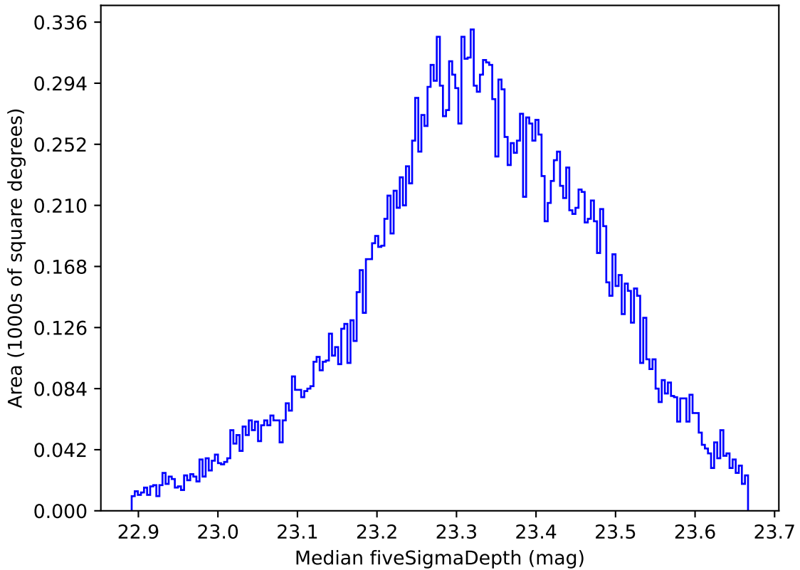
ddf_acor_sf10_lsf30_lsr20_v3.4_10yrs All sky all bands: Median fiveSigmaDepth
