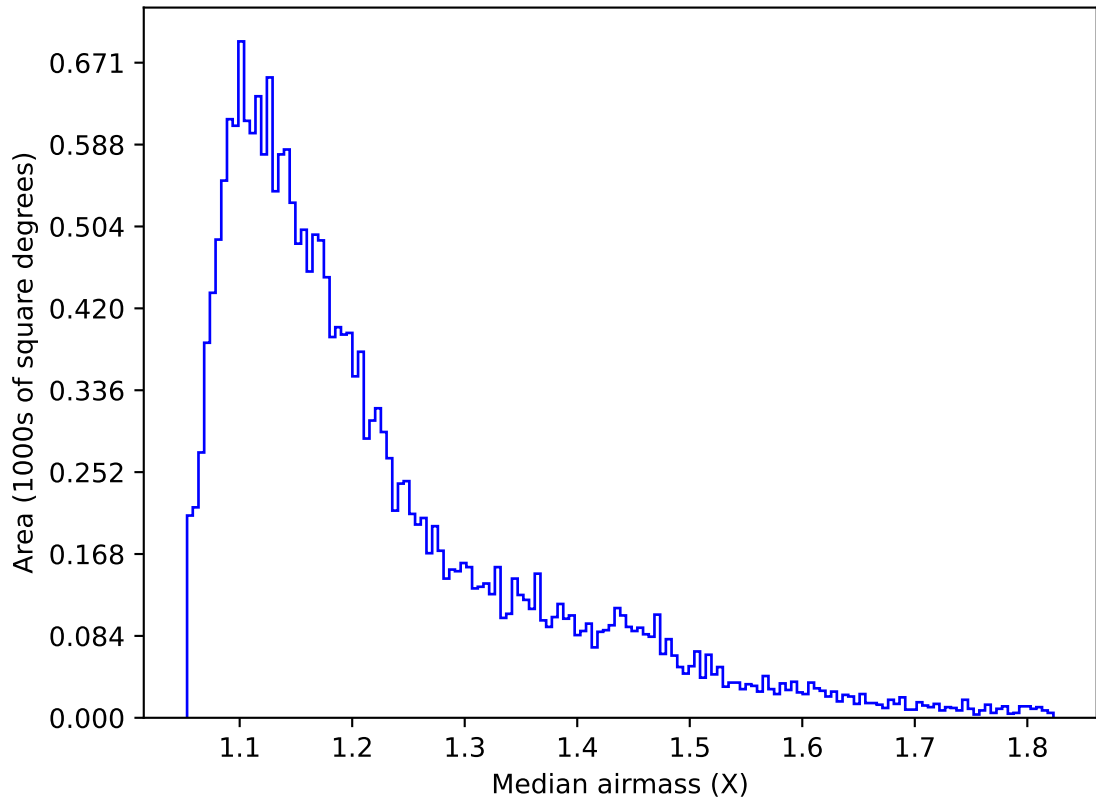
ddf_acor_sf10_lsf30_lsr20_v3.4_10yrs Yr 1 u band: Median airmass
