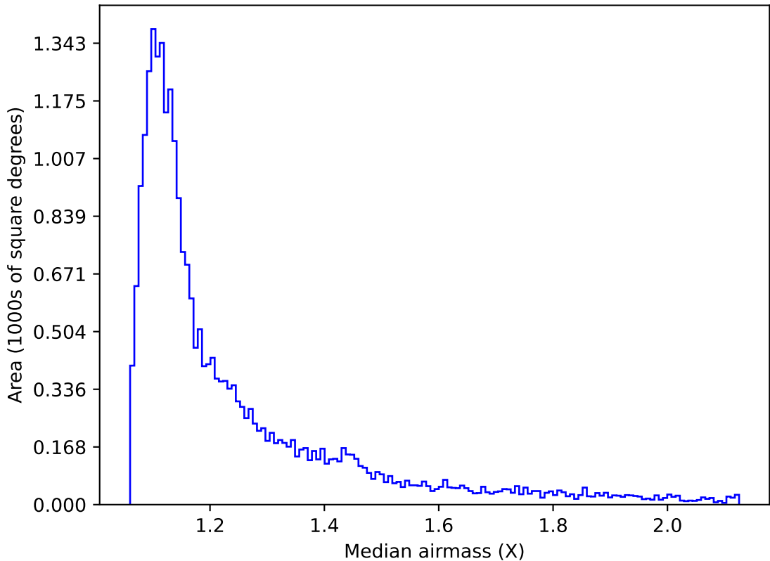
ddf_acor_sf10_lsf30_lsr20_v3.4_10yrs Yr 1 r band: Median airmass
