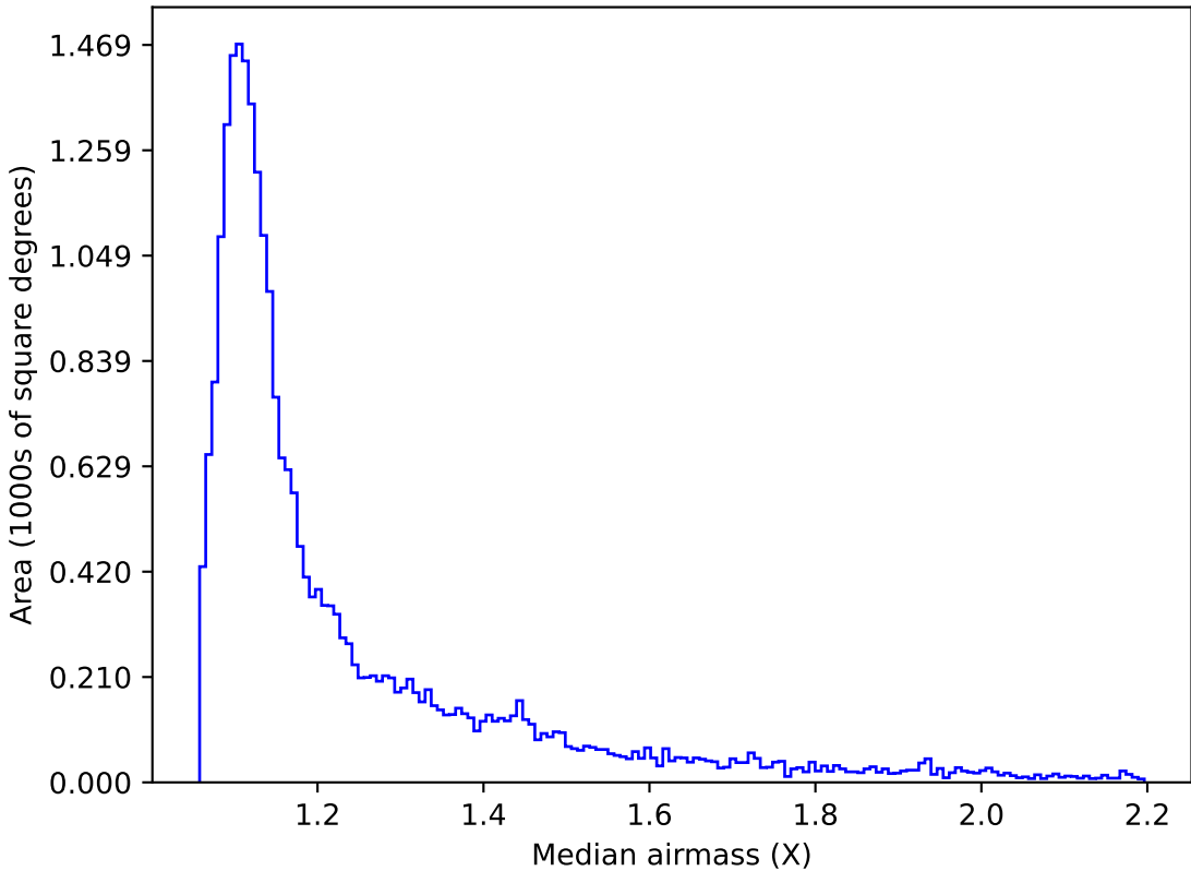
ddf_acor_sf10_lsf30_lsr20_v3.4_10yrs Yr 1 i band: Median airmass
