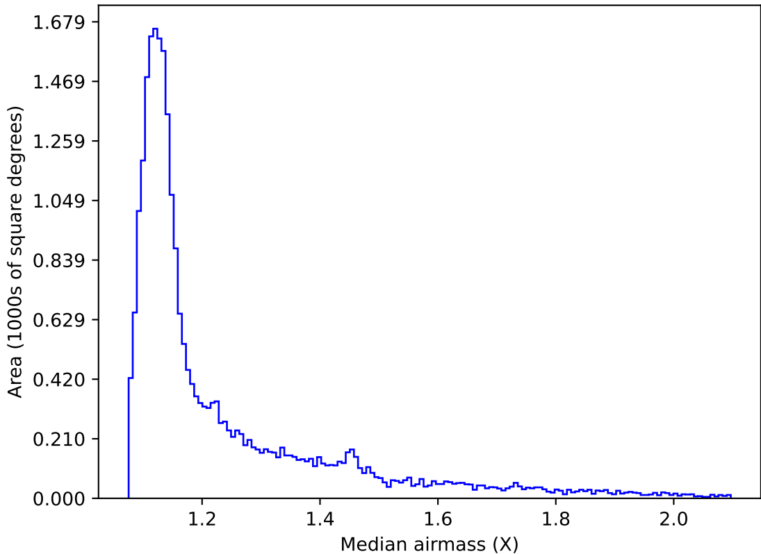
ddf_acor_sf10_lsf30_lsr20_v3.4_10yrs Yr 1 all bands: Median airmass
