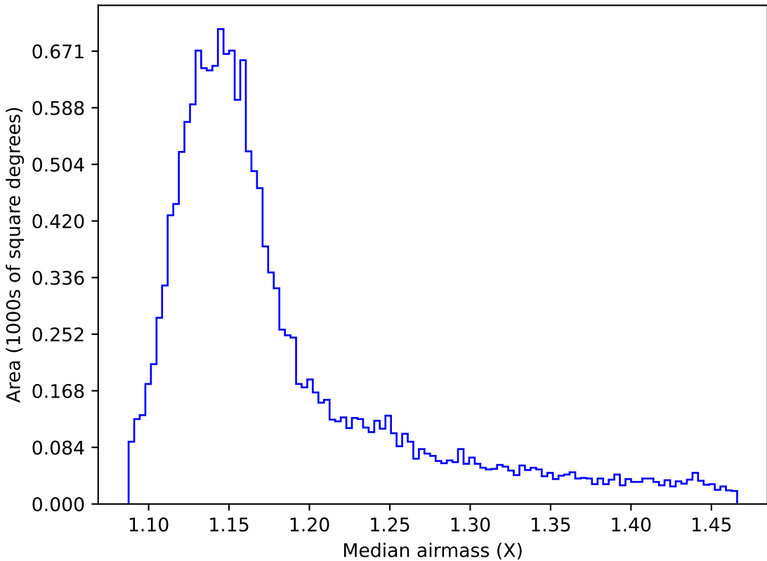
ddf_acor_sf10_lsf30_lsr20_v3.4_10yrs WFD z band: Median airmass
