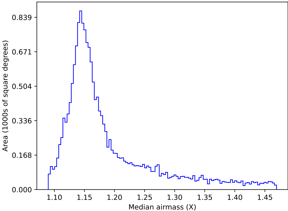
ddf_acor_sf10_ls30_lsr20_v3.4_10yrs WFD y band: Median airmass
