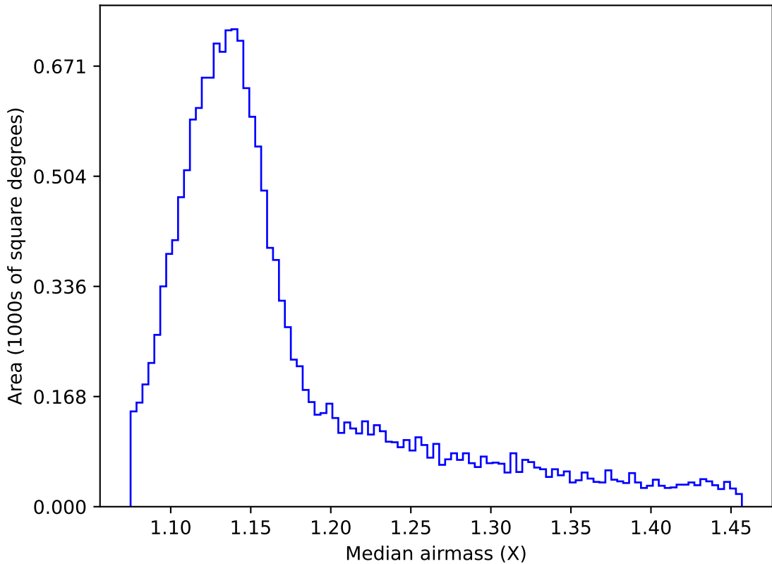
ddf_acor_sf10_lsf30_lsr20_v3.4_10yrs WFD r band: Median airmass
