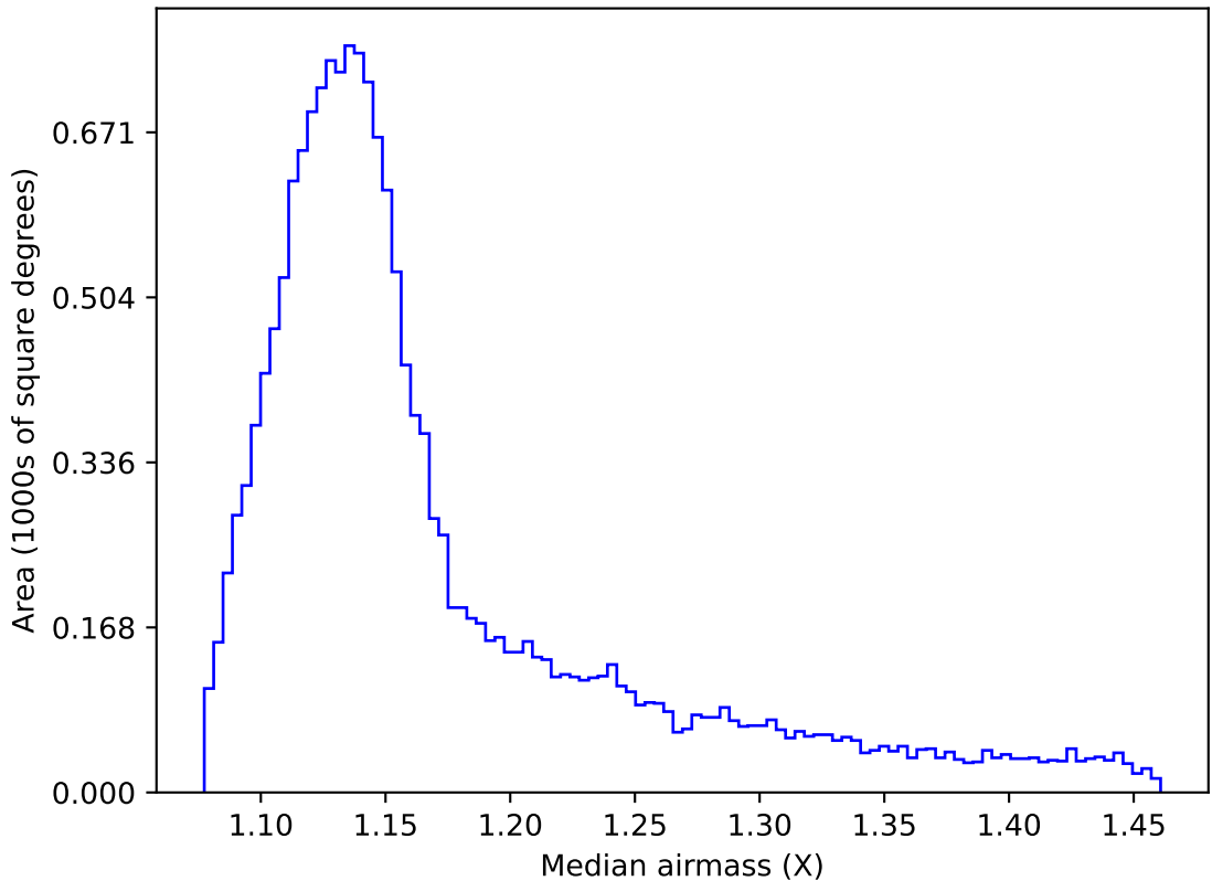
ddf_acor_sf10_lsf30_lsr20_v3.4_10yrs WFD i band: Median airmass
