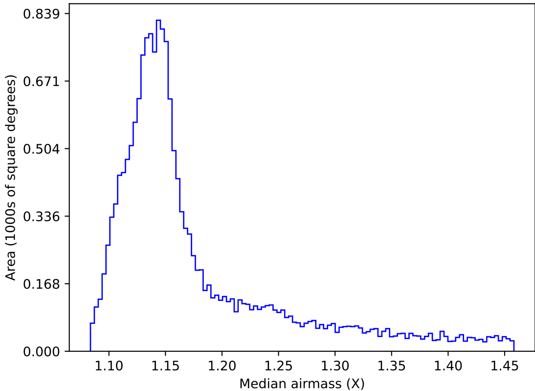
ddf_acor_sf10_lsf30_lsr20_v3.4_10yrs WFD all bands: Median airmass
