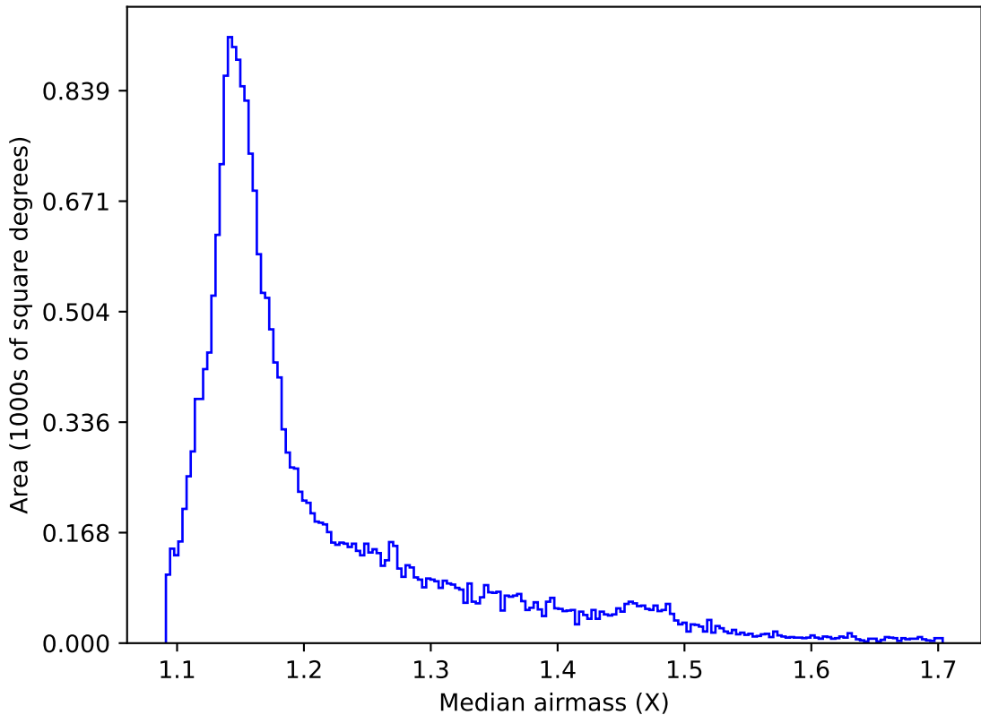
ddf_acor_sf10_lsf30_lsr20_v3.4_10yrs All sky y band: Median airmass
