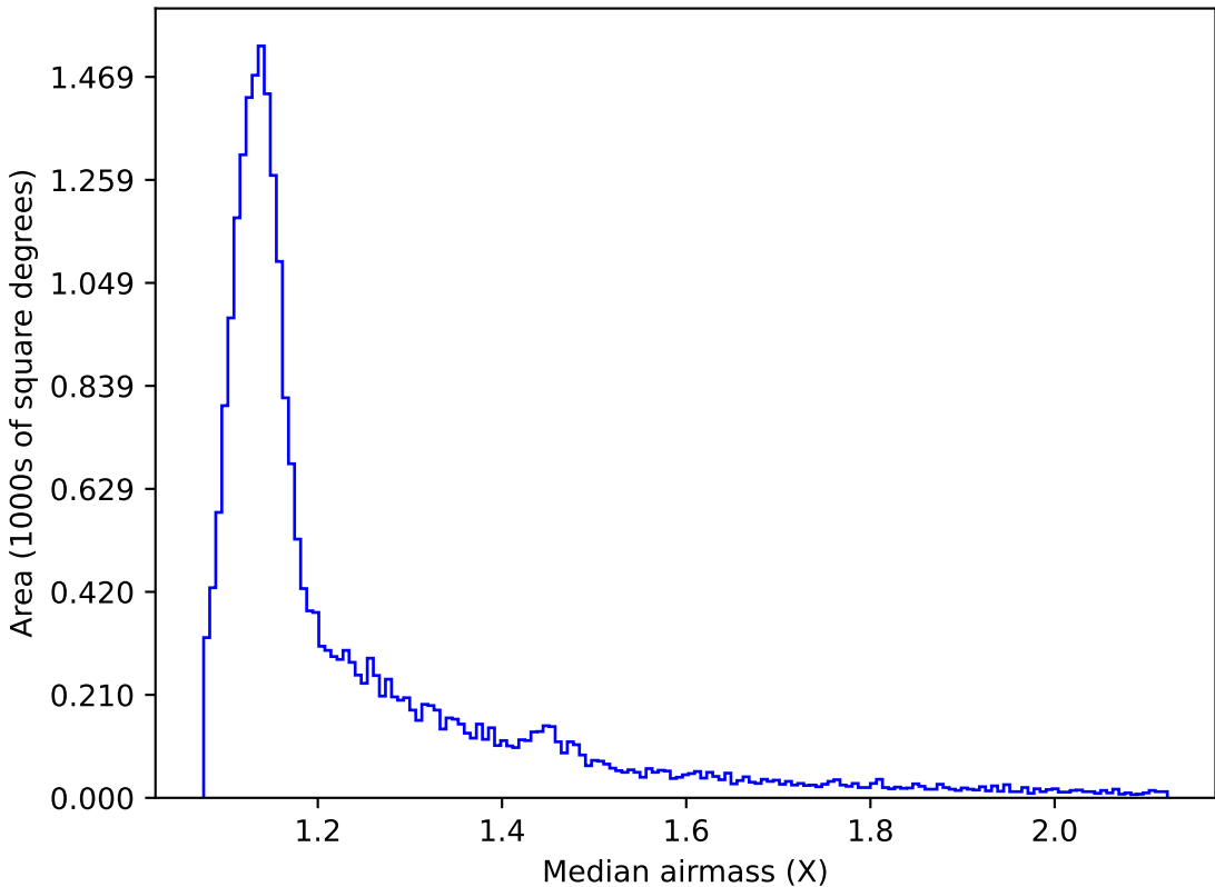
ddf_acor_sf10_lsf30_lsr20_v3.4_10yrs All sky r band: Median airmass
